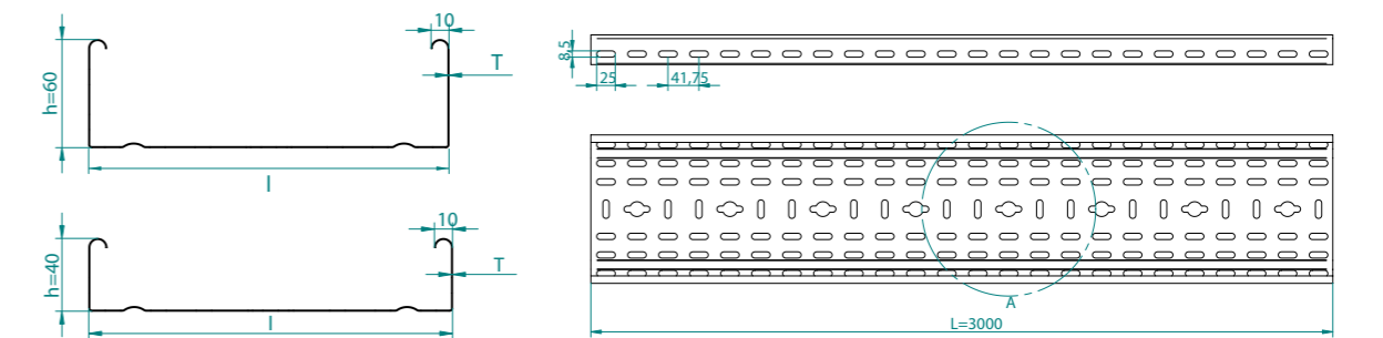
Jgheab metalic H=40mm / Cable trays H=40mm
