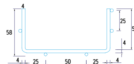
Jgheab sârmă H=60mm / Wire mesh cable trays H=60mm
